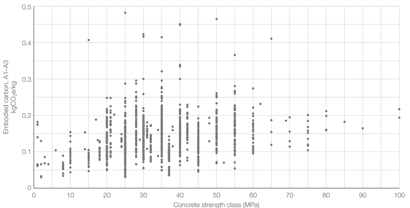
Figure 2.4: Example of possible variation in embodied carbon for concrete mixes. The concrete strength class reported is highest end in given ranges for those mixes
