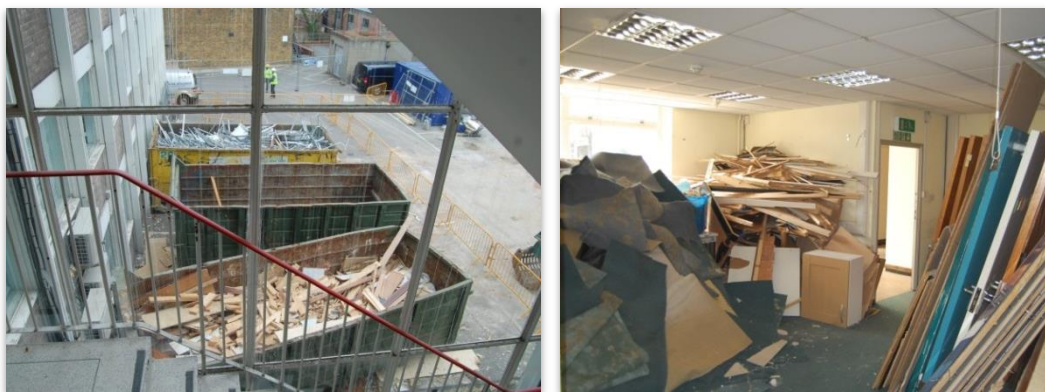
Source separation at a demolition site, Source: UEPG
